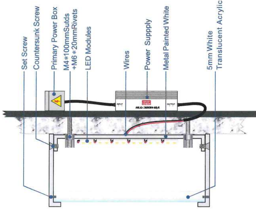
SIDE VIEW INSTALLATION DETAIL SCALE
